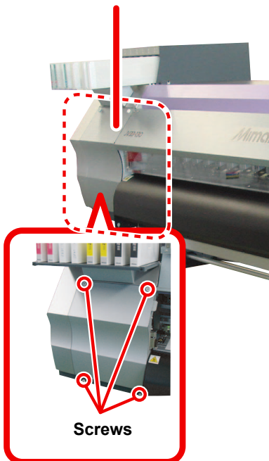
Maintenance cover
